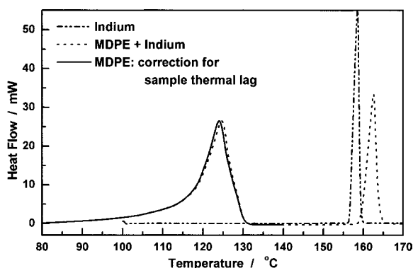
Fig. 10. Determination of the thermal resistance of a polyethylene sample (thickness=0.01 cm; area=0.3298 cm 2 ; sample mass=12.04 mg; sample resistance=23.021 °/W). All runs were obtained with temperature calibration on heating according to Eq. (13). Scanning rate=10°C/min.
