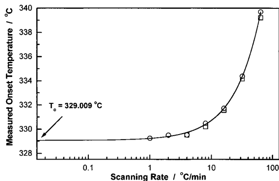
Fig. 2. Measured melting onset temperature vs. scanning rate, without calibration. Results for a lead sample with 5.055 mg and 99.99% pure, from Goodfellow. T_o is obtained from the (linear) plot of the onset temperature against the scanning rate.
