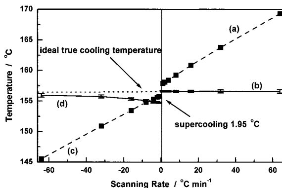
Fig. 5. Measured temperatures for indium melting and crystallization at different scanning rates (sample mass=8.143 mg). (a) heating without calibration; (b) heating with calibration according to Eq. (13); (c) cooling without calibration; (d) cooling with calibration according to Eq. (16). The ideal true cooling temperature is the temperature that should be measured if the sample analysed had no supercooling and providing all the mentioned corrections were performed.
